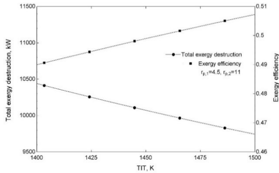
Figure 12 Total exergy destruction and exergy efficiency vs. TIT.
