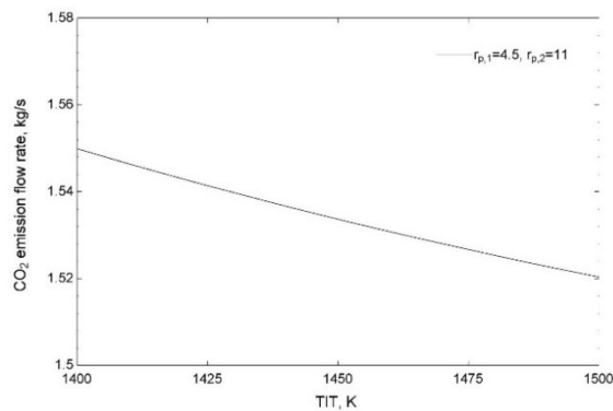
Figure 9 CO 2 emissions vs. a) r_{p1} , b) r_{p2} , and c) TIT.
