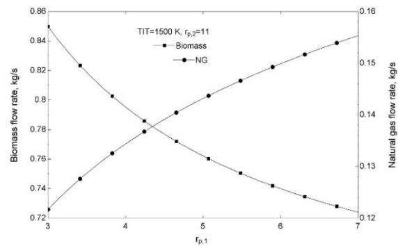
Figure 4 Biomass and the natural gas flow rate vs. r_{p1} .
