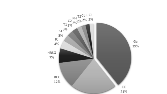
Figure 15 The contribution of the exergy destruction rates within CCIR components (except Pu).
