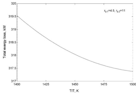
Figure 13 Total exergy loss versus TIT.
